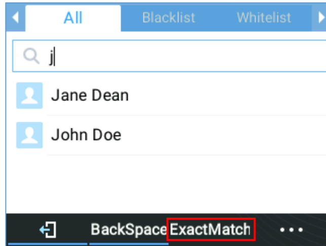
Figure 68: ExactMatch
